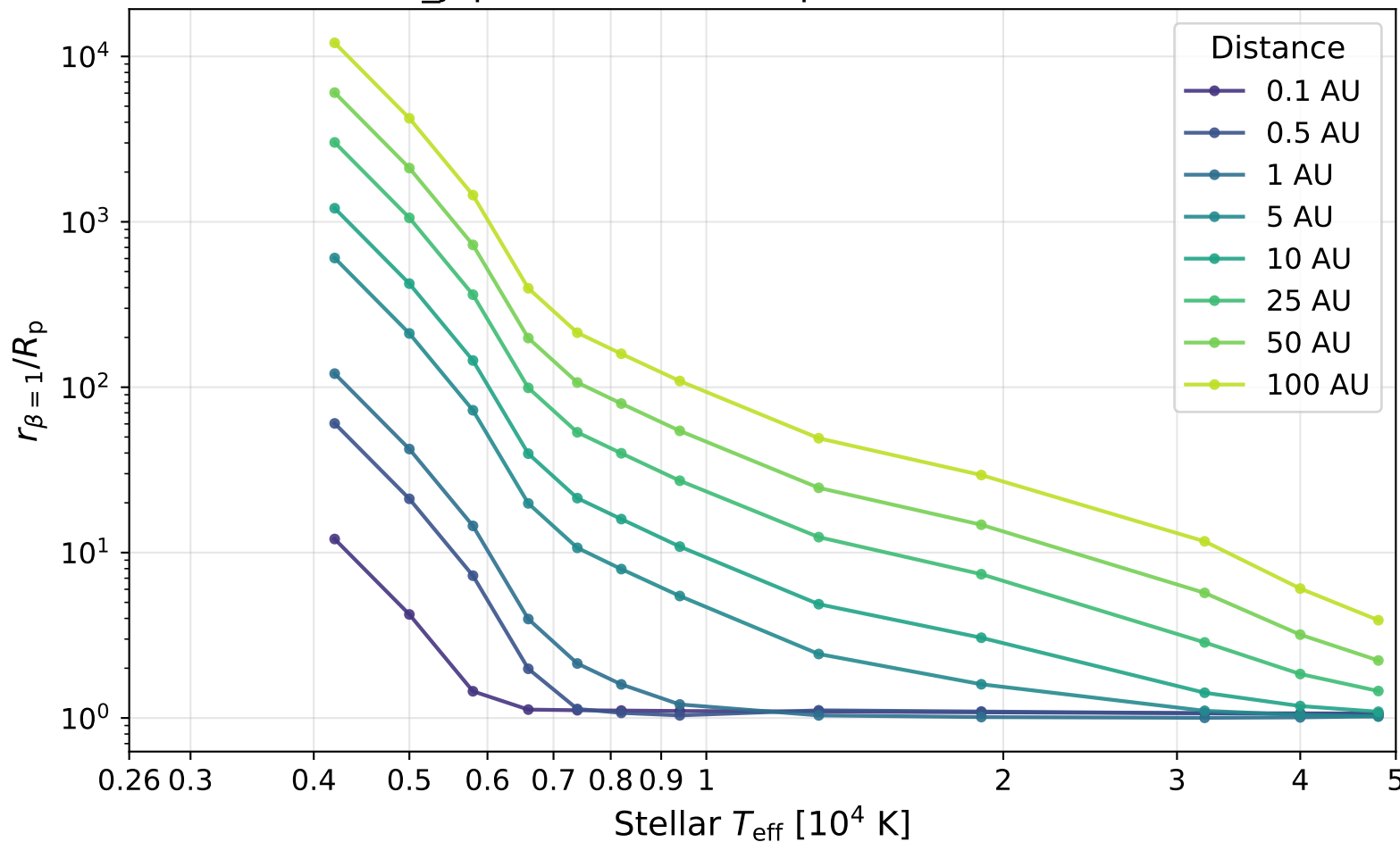
hot_jupiter: Na I at multiple orbital distances
